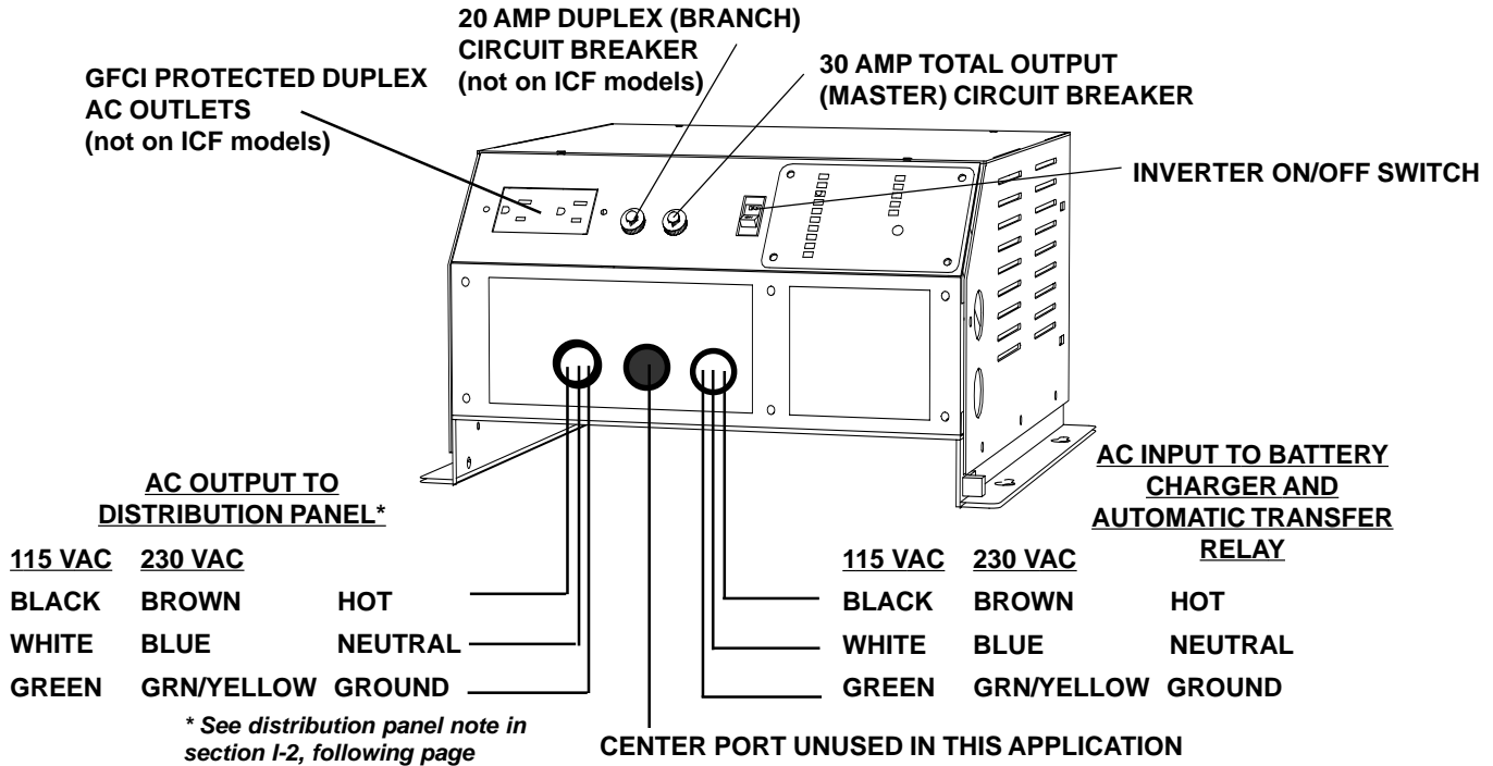
FIGURE 3: AC Input and Output Wiring
