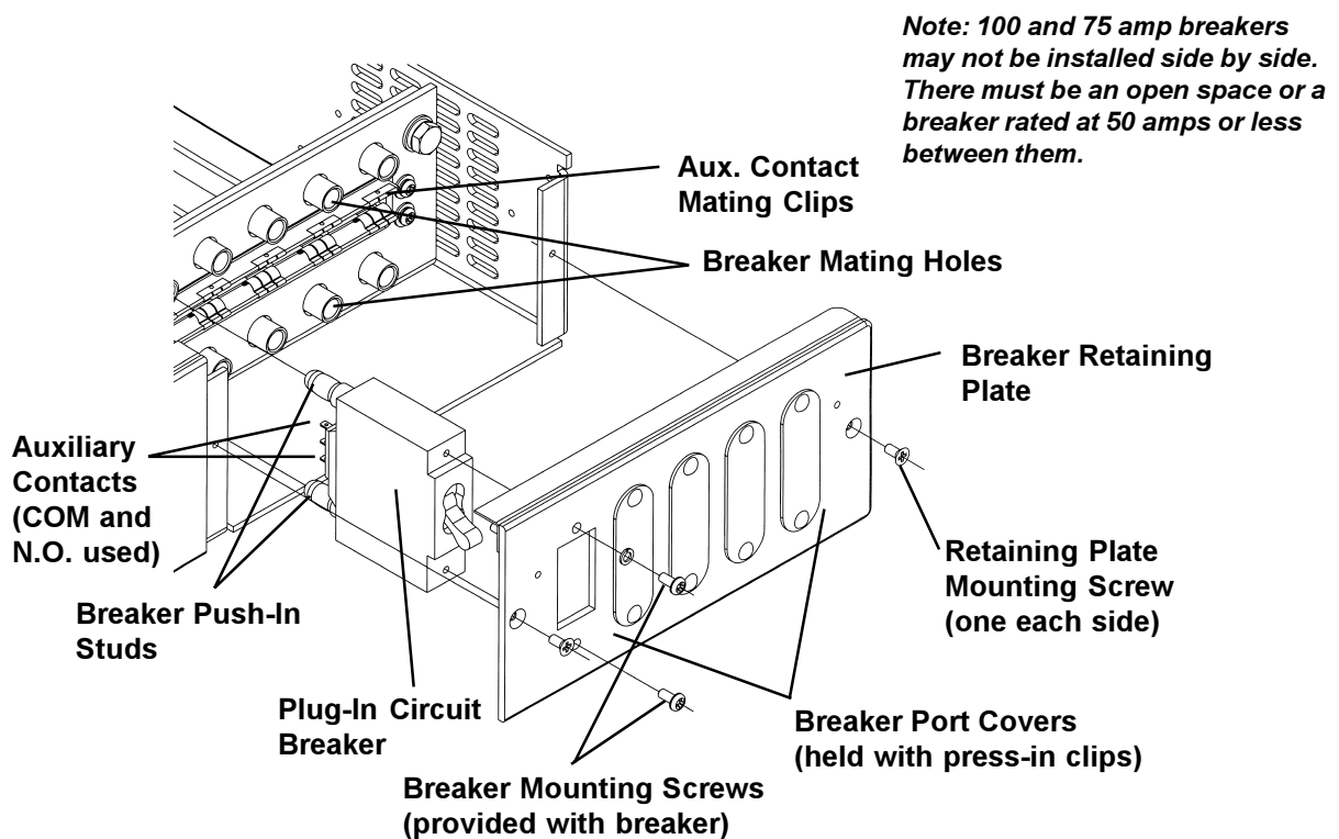
FIGURE 7: Circuit Breaker Installation
