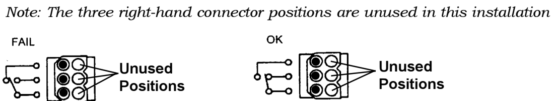
FIGURE 6: d.c. "FAIL" and d.c. "OK" Summary Alarm Contact Positions (as viewed from rear of chassis)
