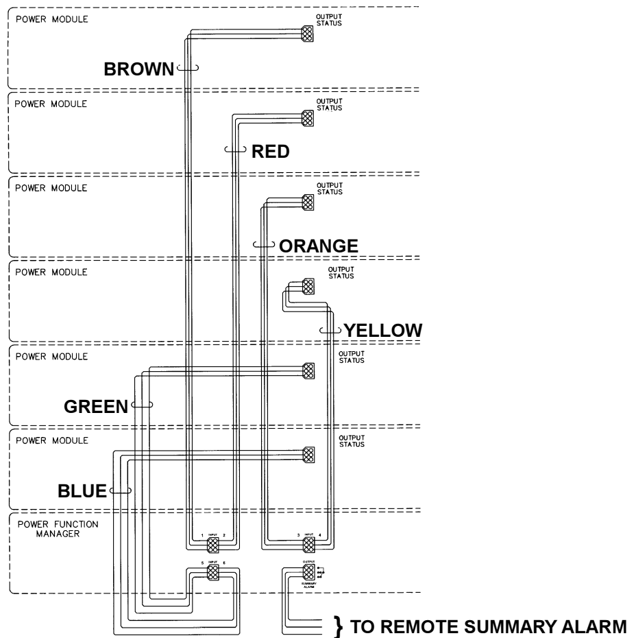
FIGURE 5: Typical Status Contact and Summary Alarm Wiring
